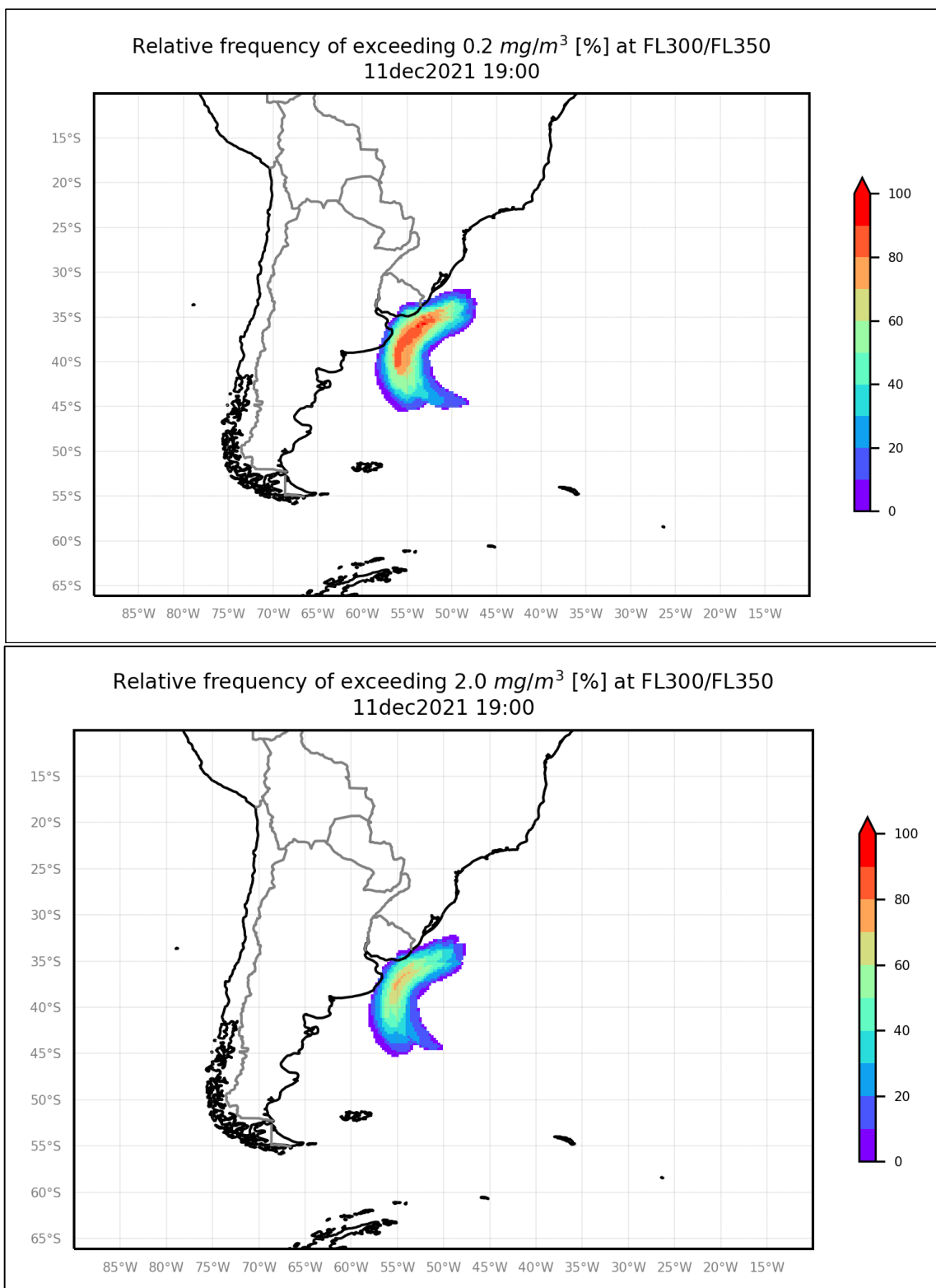
Figure 8. Visualized examples of QVA grid point probability information from FL 300 to FL 350. Upper frame is the probability of exceeding 0.2 mg/m³. Lower frame is the probability of exceeding 2 mg/m³.
